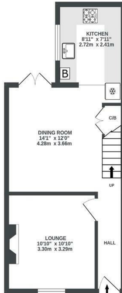
GROUND FLOOR 386 sq.ft. (35.9 sq.m.) approx.
